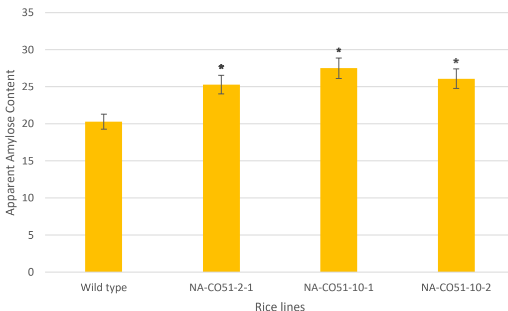
Fig. 1. Apparent amylose content [%]
