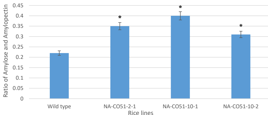
Fig. 4. Ratio of Amylose/Amylopectin
